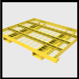
FLOW-THROUGH TOP
