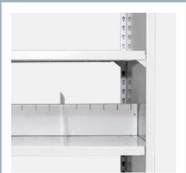
Double-Face Shelving Fixed Middle Shelf and Center Stop with Dividers on Lower Shelf
